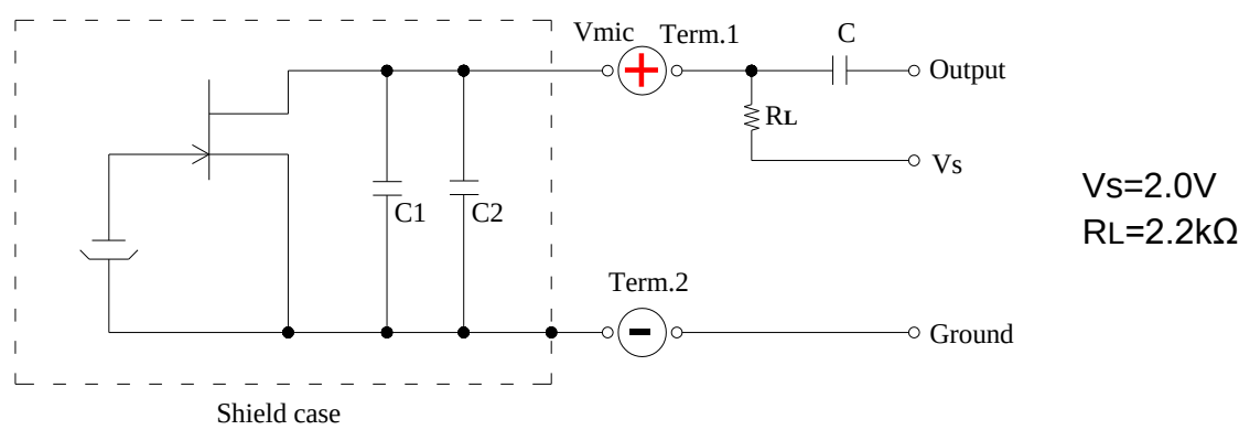
Fig. 5-1 Schematic Diagram
