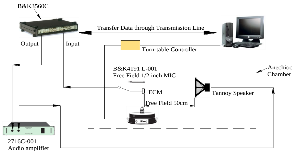
Fig. 6-1 Measurement System Setup
