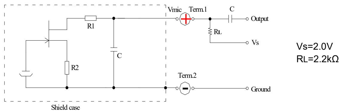
Fig. 5-1 Schematic Diagram
