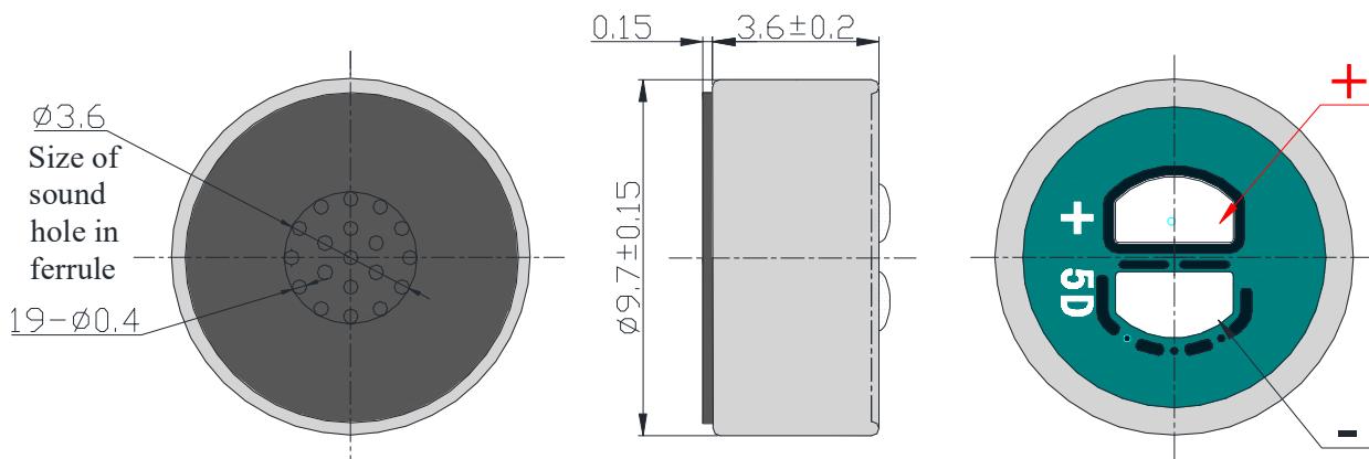
Fig. 7-1 Microphone Capsule
