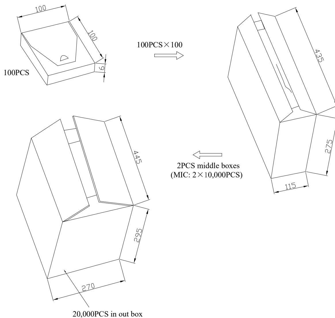
Fig. 9-1 Packaging
