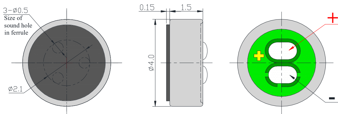
Fig. 7-1 Microphone capsule
