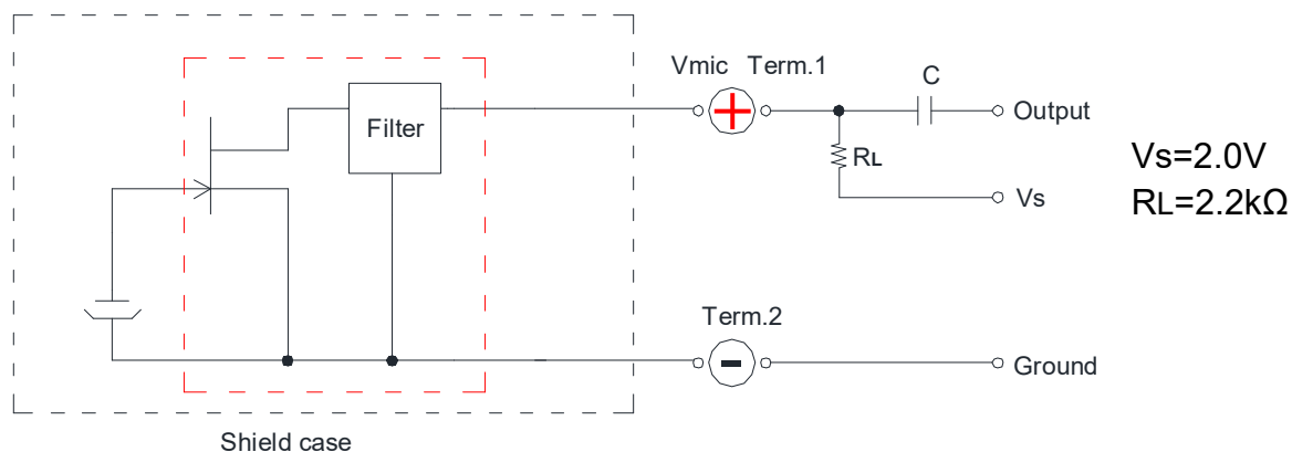
Fig. 5-1 Schematic Diagram
