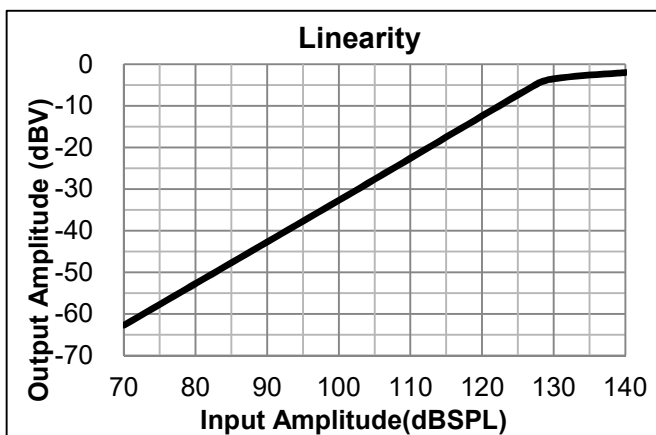
Fig. 6 Linearity
