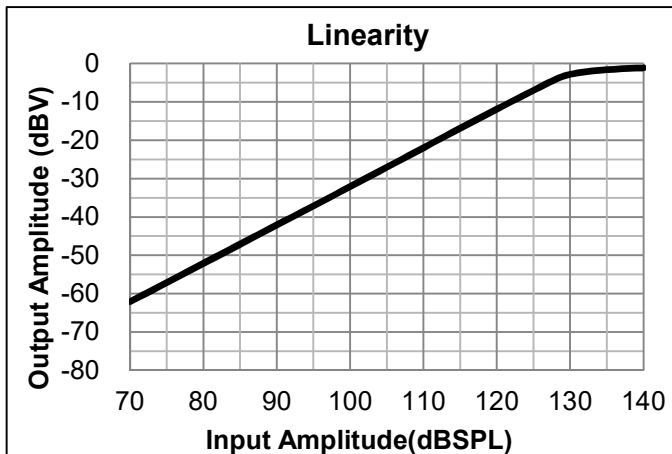
Fig. 6 Linearity
