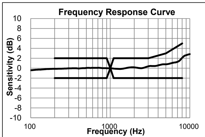
Fig.2 Frequency response curve normalized to 1KHz
