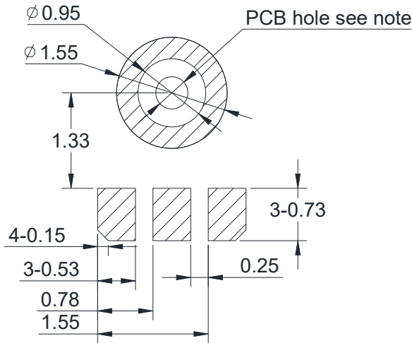
Example Land Pattern
