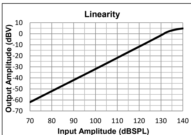
Fig. 6 Linearity
