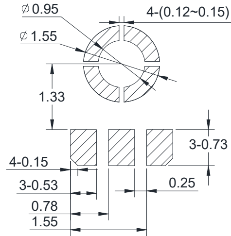
Example Solder Stencil Pattern
