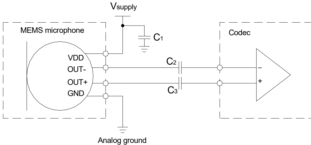
Fig. 9 Typical Application Circuit
