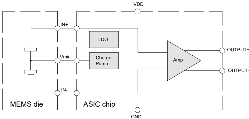
Fig. 1 Microphone block diagram
