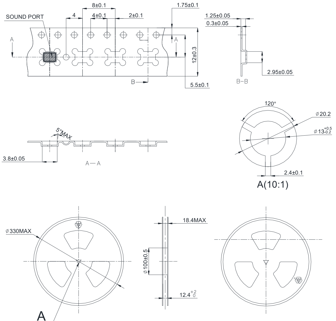
Fig. 14 Packaging
