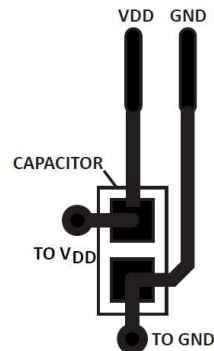
Fig. 12 Recommended Power Supply Decoupling Capacitor Layout
